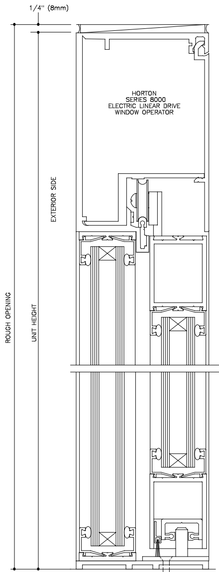
VERTICAL SECTION SCALE: FULL (1)
