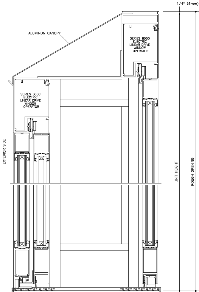
VERTICAL SECTION SCALE: FULL 1 WINDOW SHOWN IN OPEN POSITION
