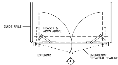
FLOOR PLAN NOT TO SCALE (3)
