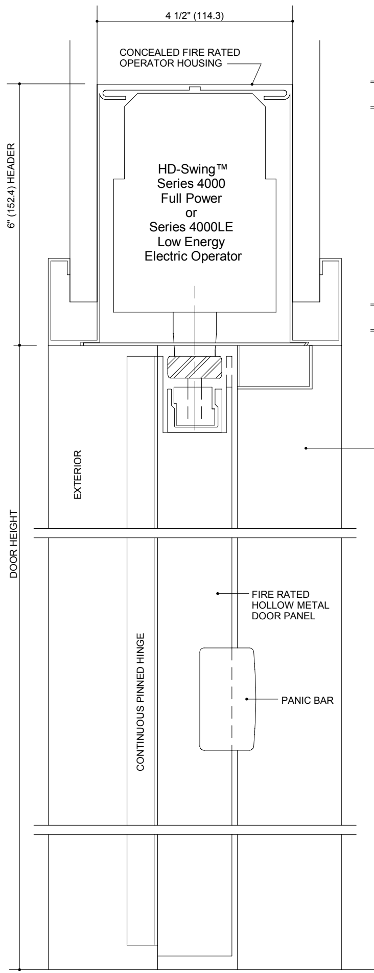
VERTICAL SECTION FULL SCALE 1
