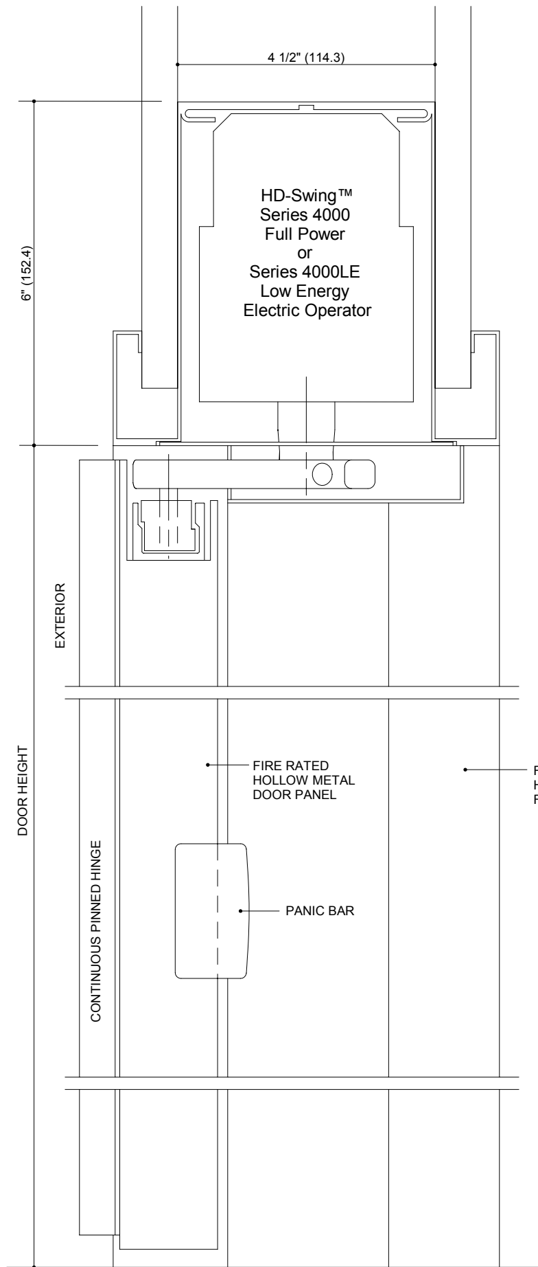
VERTICAL SECTION FULL SCALE 1
