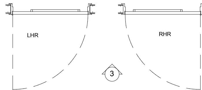
FLOOR PLANS NOT TO SCALE 4
