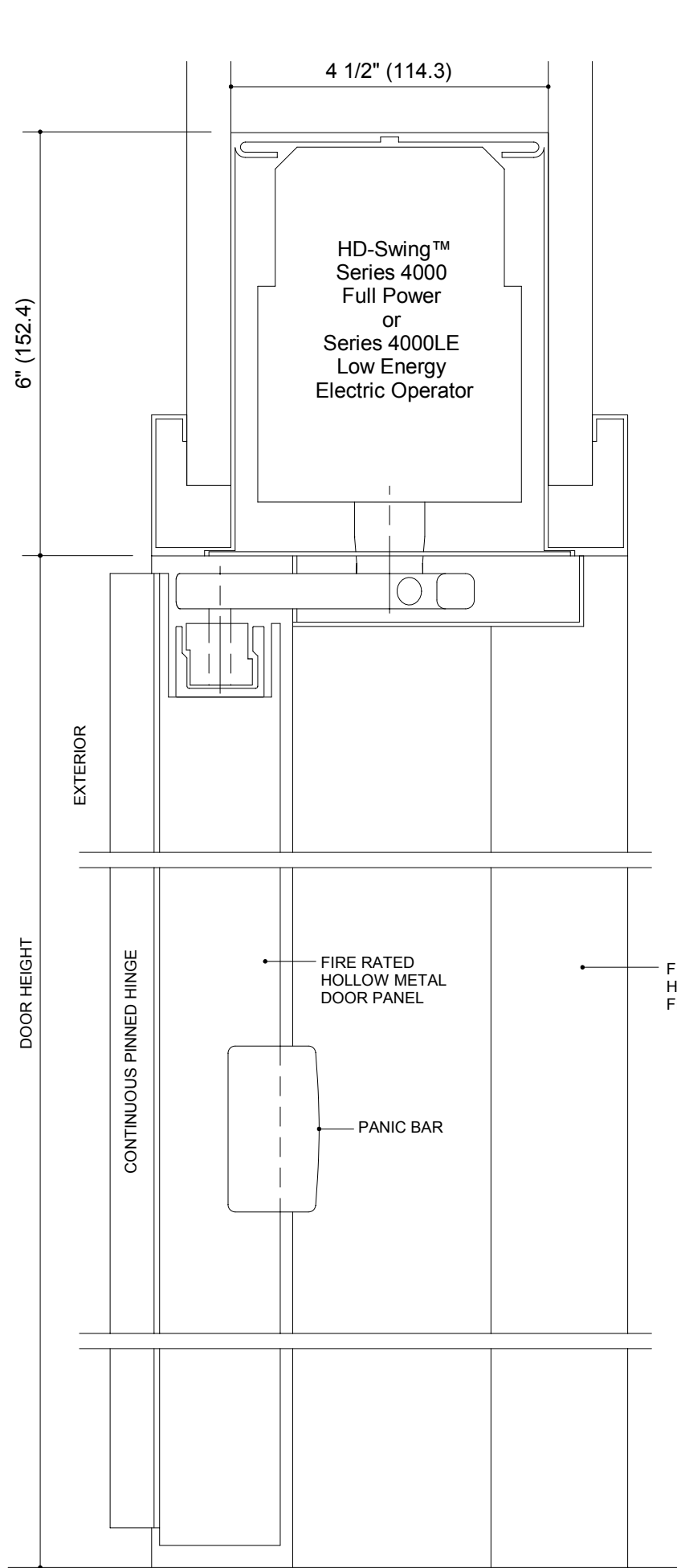
VERTICAL SECTION FULL SCALE 1
