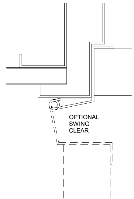
HORIZONTAL SECTION FULL SCALE - LRH SHOWN RHR OPPOSITE 2
