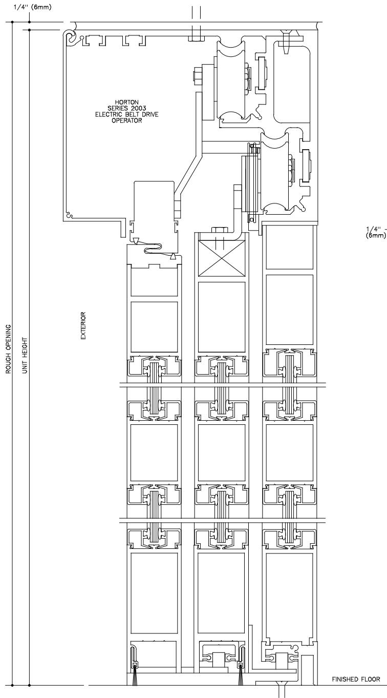
VERTICAL SECTION FULL SCALE 1 DOOR SHOWN IN OPEN POSITION
