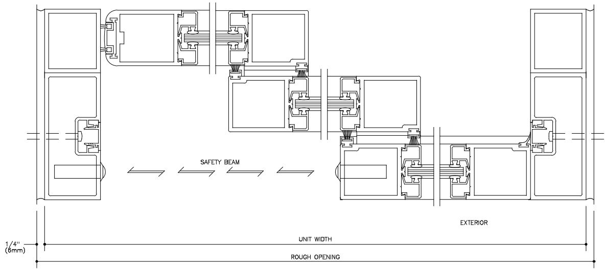
HORIZONTAL SECTION FULL SCALE 2
