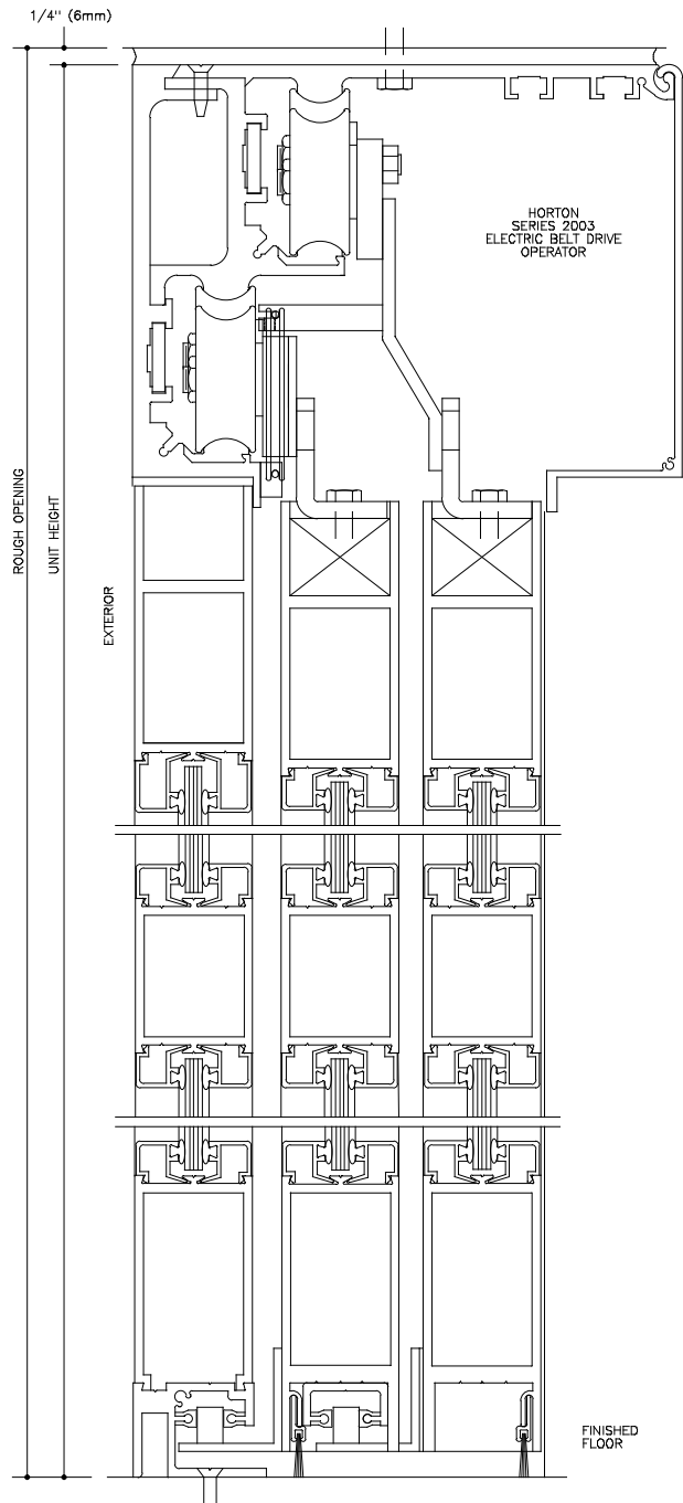
VERTICAL SECTION FULL SCALE DOOR SHOWN IN OPEN POSITION
