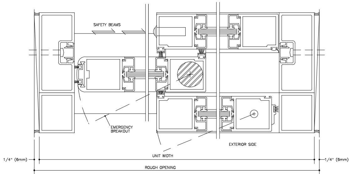
HORIZONTAL SECTION FULL SCALE (2)
