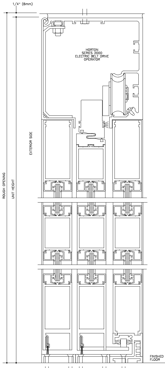
VERTICAL SECTION FULL SCALE (1) DOOR SHOWN IN OPEN POSITION
