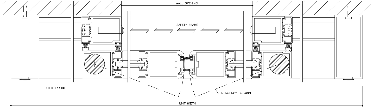
HORIZONTAL SECTION FULL SCALE 2
