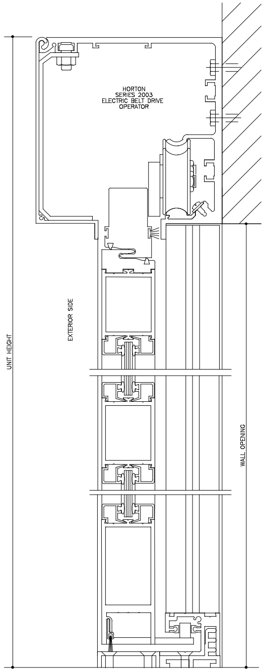
VERTICAL SECTION FULL SCALE 1 DOOR SHOWN IN OPEN POSITION
