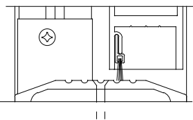
THRESHOLD SECTION FULL SCALE DOOR SHOWN IN CLOSED POSITION
