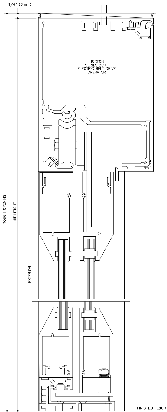
VERTICAL SECTION FULL SCALE 1 DOOR SHOWN IN OPEN POSITION
