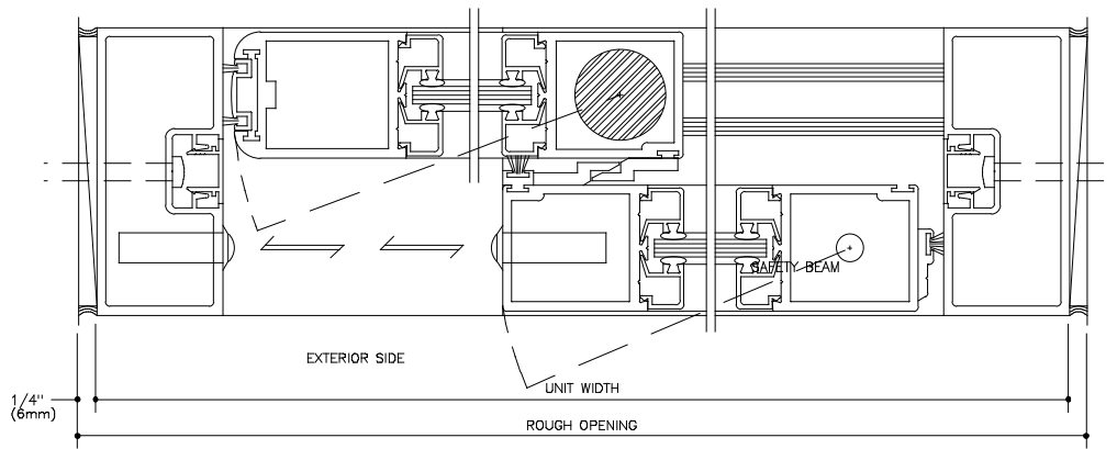
HORIZONTAL SECTION FULL SCALE 2
