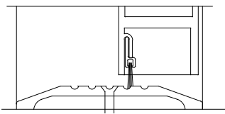
THRESHOLD SECTION FULL SCALE 3 DOOR SHOWN IN CLOSED POSITION
