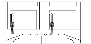
THRESHOLD SECTION FULL SCALE DOOR SHOWN IN CLOSED POSITION
