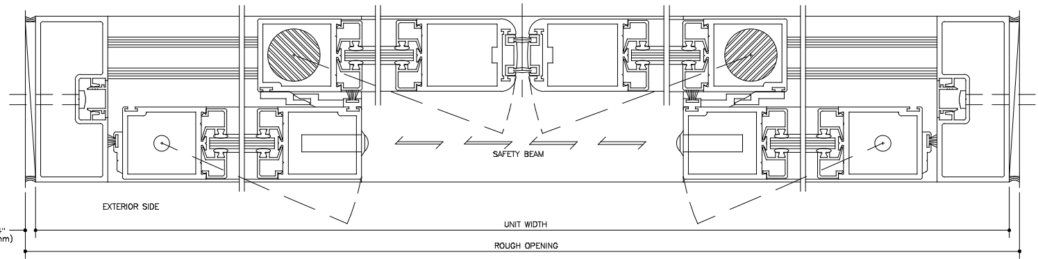
HORIZONTAL SECTION FULL SCALE
