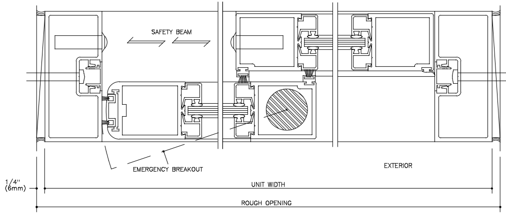
HORIZONTAL SECTION FULL SCALE
