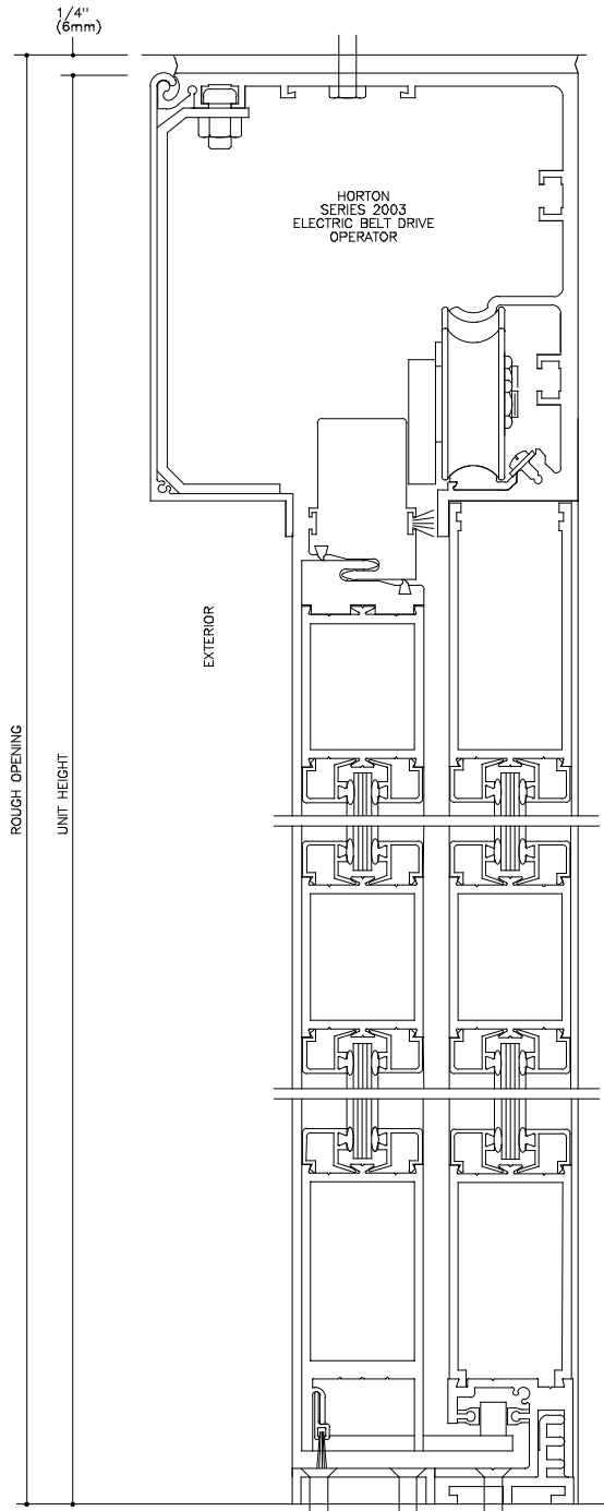
VERTICAL SECTION FULL SCALE DOOR SHOWN IN OPEN POSITION
