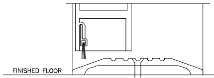
THRESHOLD SECTION FULL SCALE
