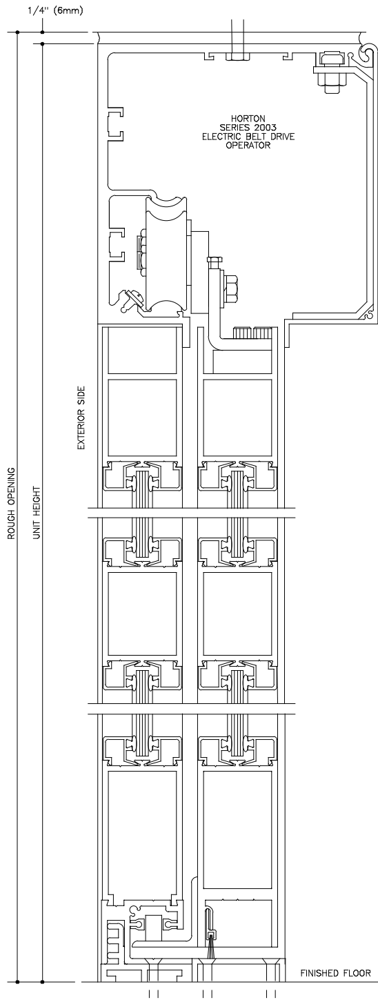
VERTICAL SECTION FULL SCALE DOOR SHOWN IN OPEN POSITION 1
