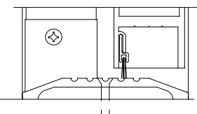
THRESHOLD SECTION FULL SCALE DOOR SHOWN IN CLOSED POSITION
