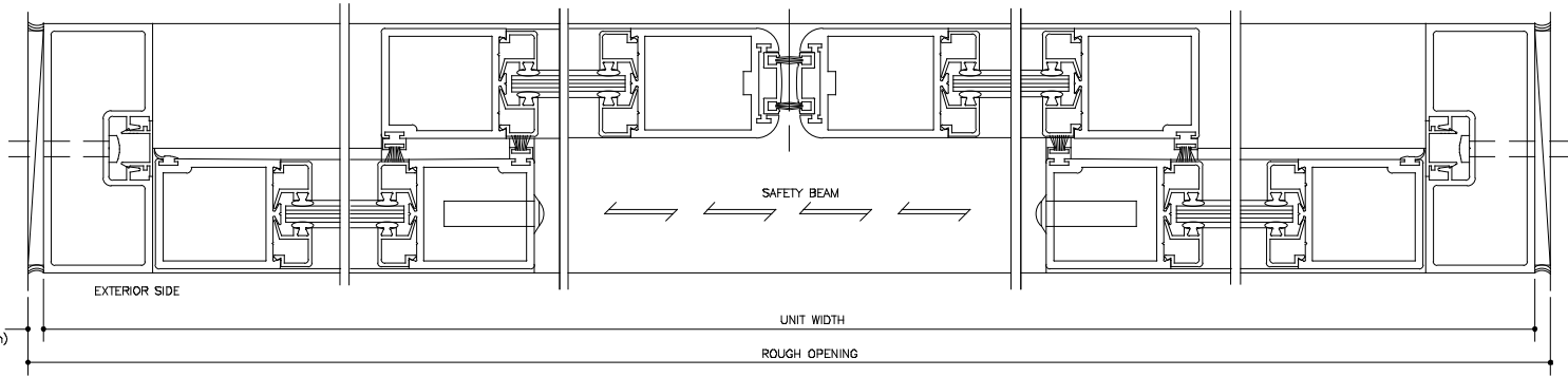
HORIZONTAL SECTION FULL SCALE
