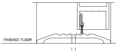
THRESHOLD SECTION FULL SCALE 3 DOOR SHOWN IN CLOSED POSITION
