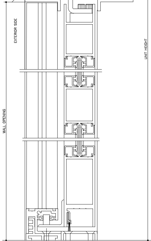
VERTICAL SECTION FULL SCALE 1 DOOR SHOWN IN OPEN POSITION
