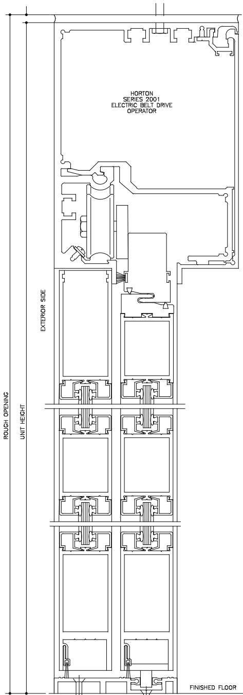
VERTICAL SECTION FULL SCALE DOOR SHOWN IN OPEN POSITION
