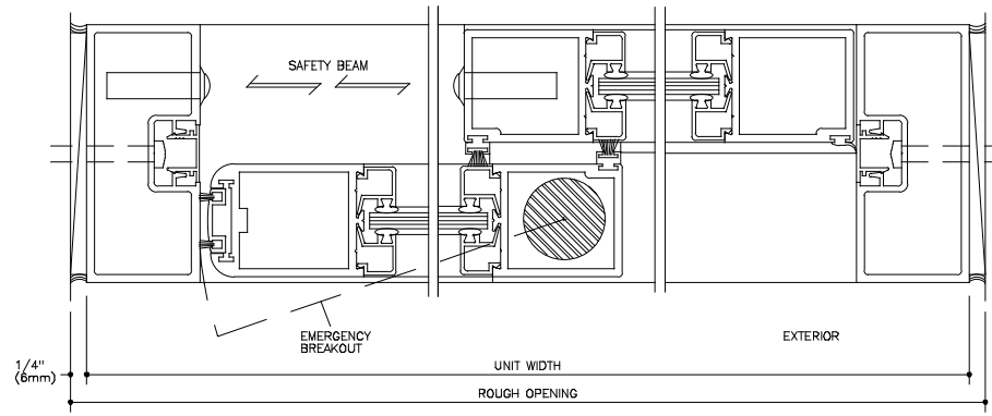
HORIZONTAL SECTION FULL SCALE
