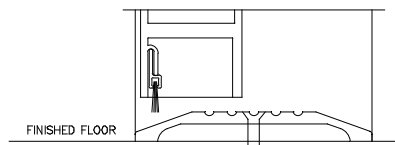
THRESHOLD SECTION FULL SCALE
