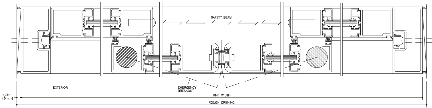
HORIZONTAL SECTION FULL SCALE
