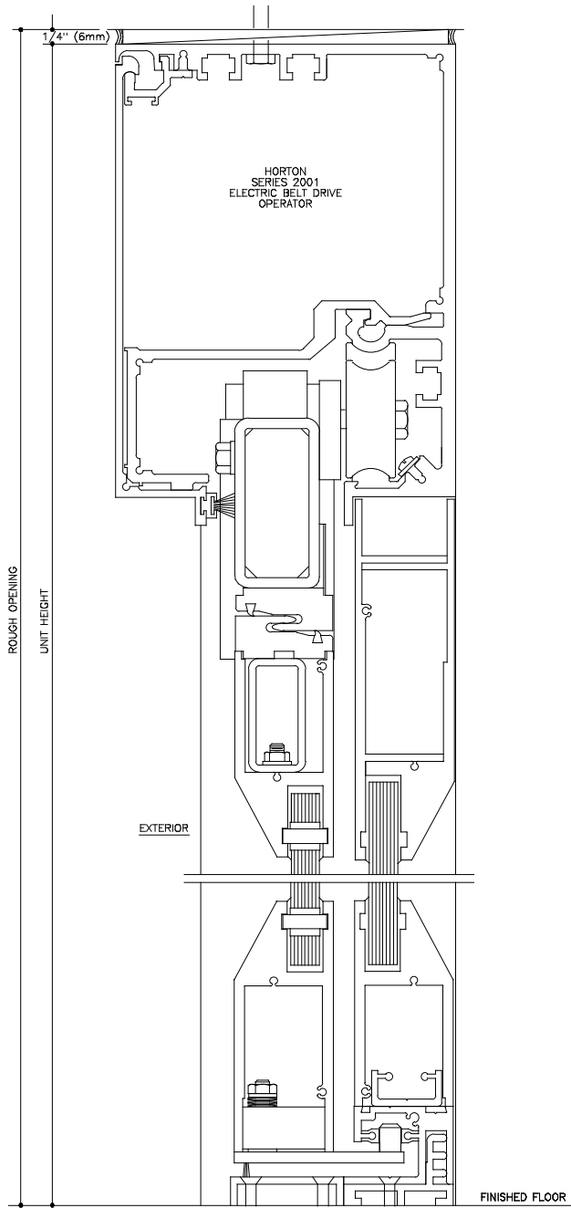
VERTICAL SECTION FULL SCALE 1 DOOR SHOWN IN OPEN POSITION
