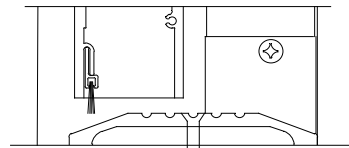
THRESHOLD SECTION FULL SCALE 3 DOOR SHOWN IN CLOSED POSITION
