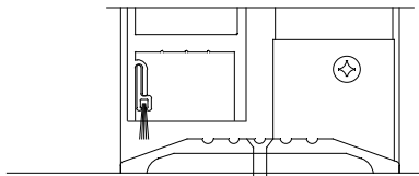
STANDARD 4" (102mm) THRESHOLD
