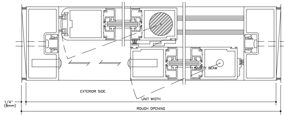
HORIZONTAL SECTION FULL SCALE 2
