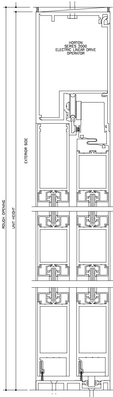
VERTICAL SECTION FULL SCALE DOOR SHOWN IN OPEN POSITION
