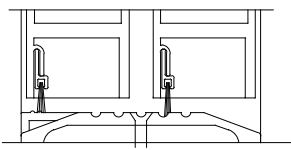
THRESHOLD SECTION FULL SCALE DOOR SHOWN IN CLOSED POSITION
