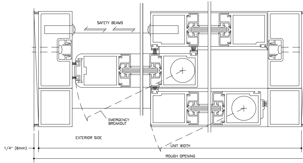
HORIZONTAL SECTION FULL SCALE
