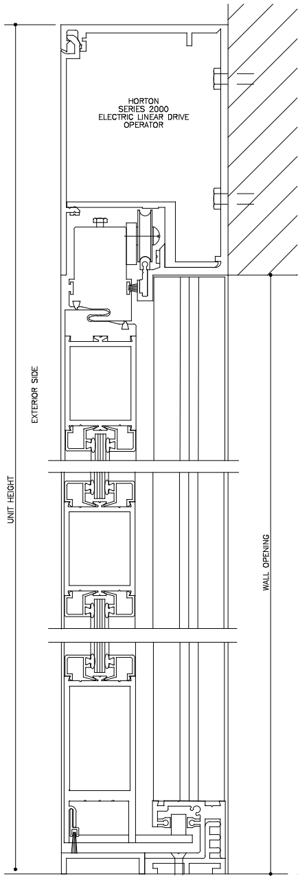
VERTICAL SECTION FULL SCALE DOOR SHOWN IN OPEN POSITION
