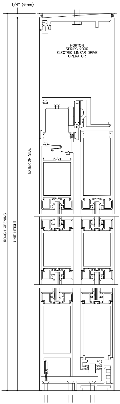
VERTICAL SECTION FULL SCALE 1 DOOR SHOWN IN OPEN POSITION
