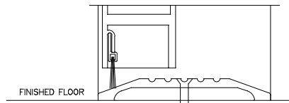
THRESHOLD SECTION FULL SCALE 3 DOOR SHOWN IN CLOSED POSITION
