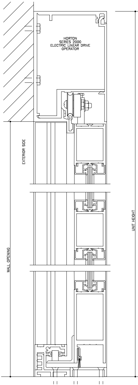
VERTICAL SECTION FULL SCALE 1 DOOR SHOWN IN OPEN POSITION
