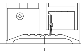
THRESHOLD SECTION FULL SCALE 3 DOOR SHOWN IN CLOSED POSITION
