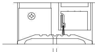
THRESHOLD SECTION FULL SCALE DOOR SHOWN IN CLOSED POSITION
