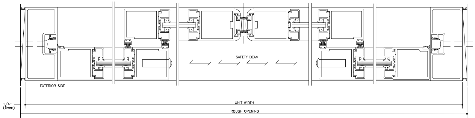
HORIZONTAL SECTION FULL SCALE
