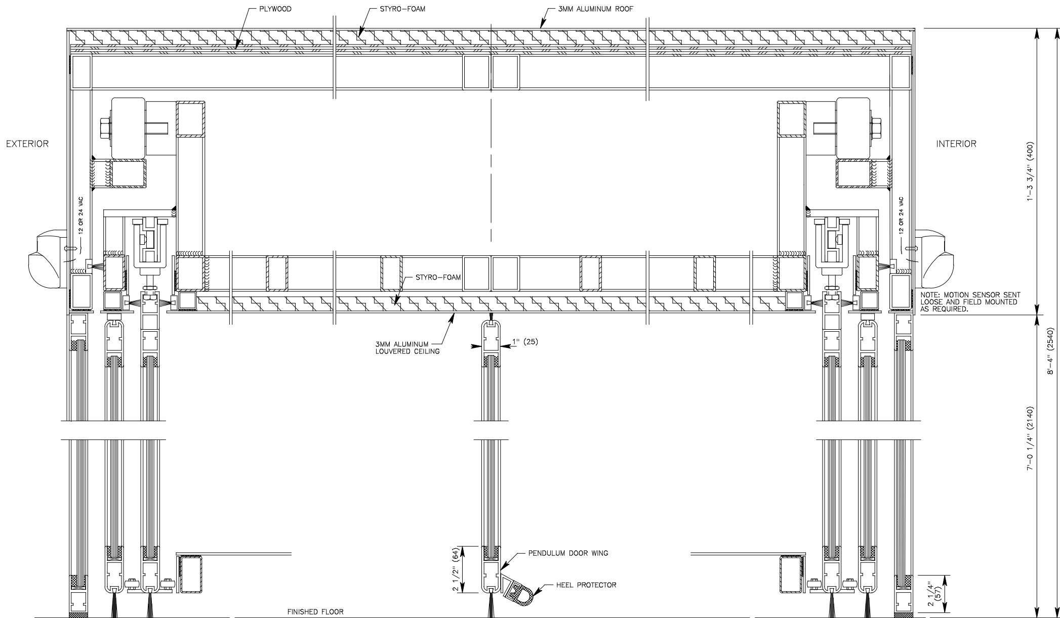
VERTICAL SECTION 1/4 SCALE
