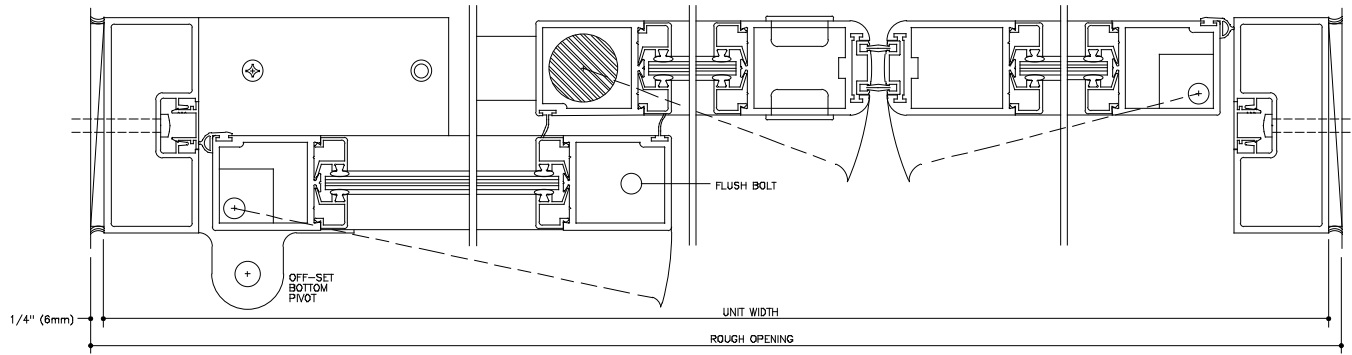
HORIZONTAL SECTION FULL SCALE
