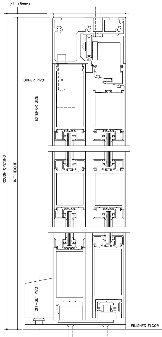
VERTICAL SECTION FULL SCALE DOOR SHOWN IN OPEN POSITION
