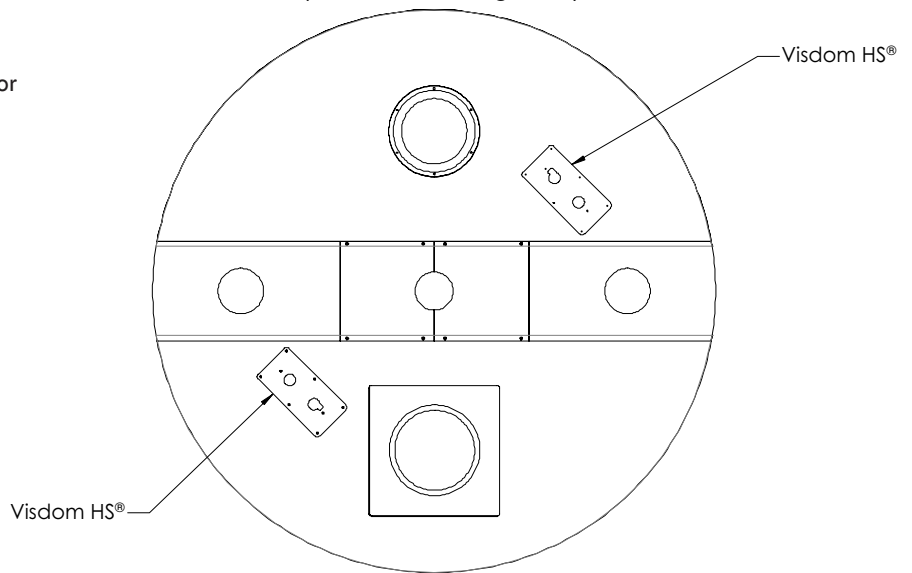
Typical Revolving Door Ceiling Installation (Reflected Ceiling View)
