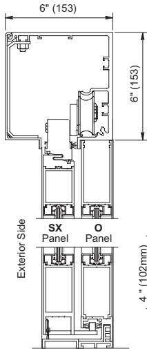
Vertical Section
