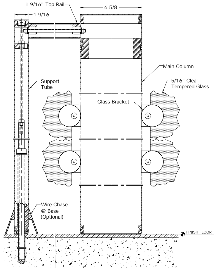
3 Vertical Sections
