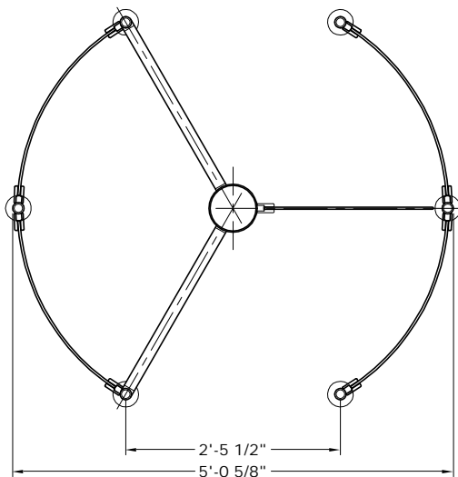
2 Plan View
